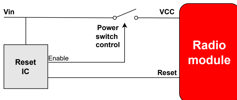
Figure 36: Reset IC
