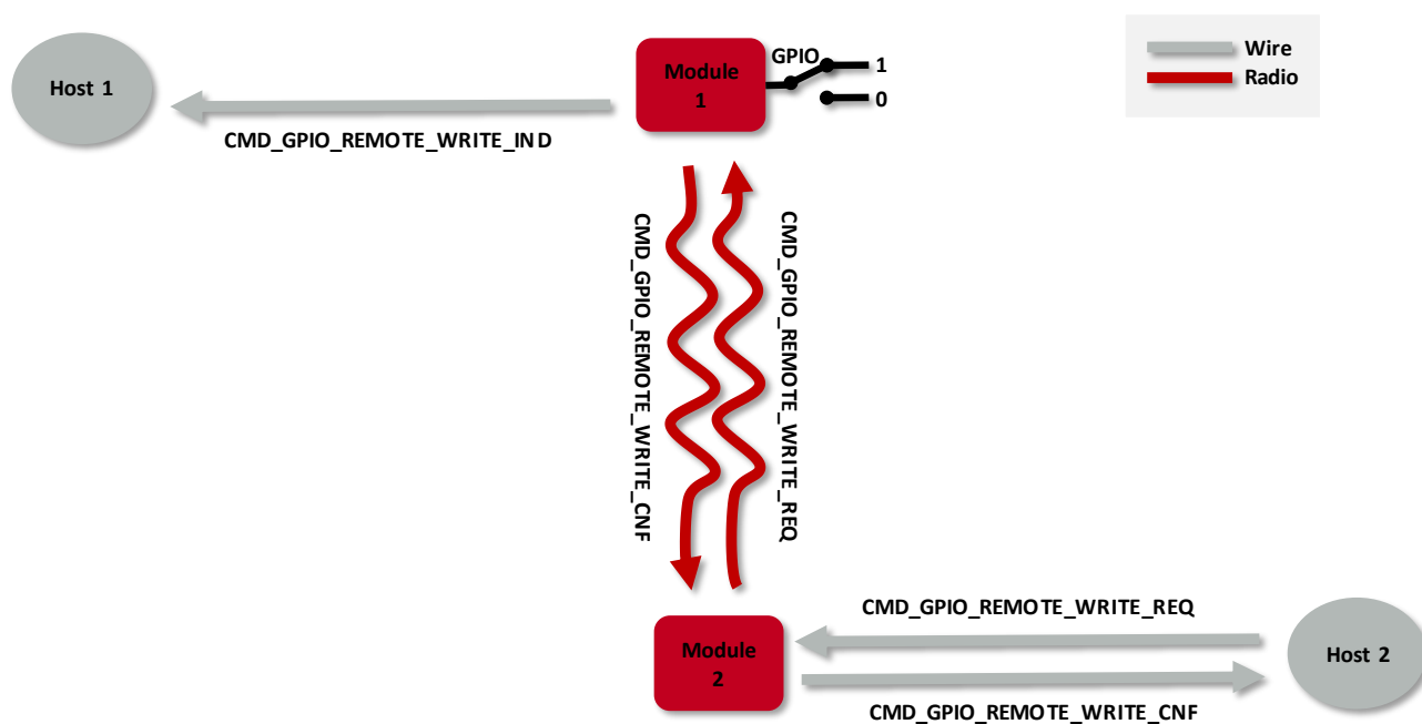
Figure 19: Set the output value of a GPIO via remote device
