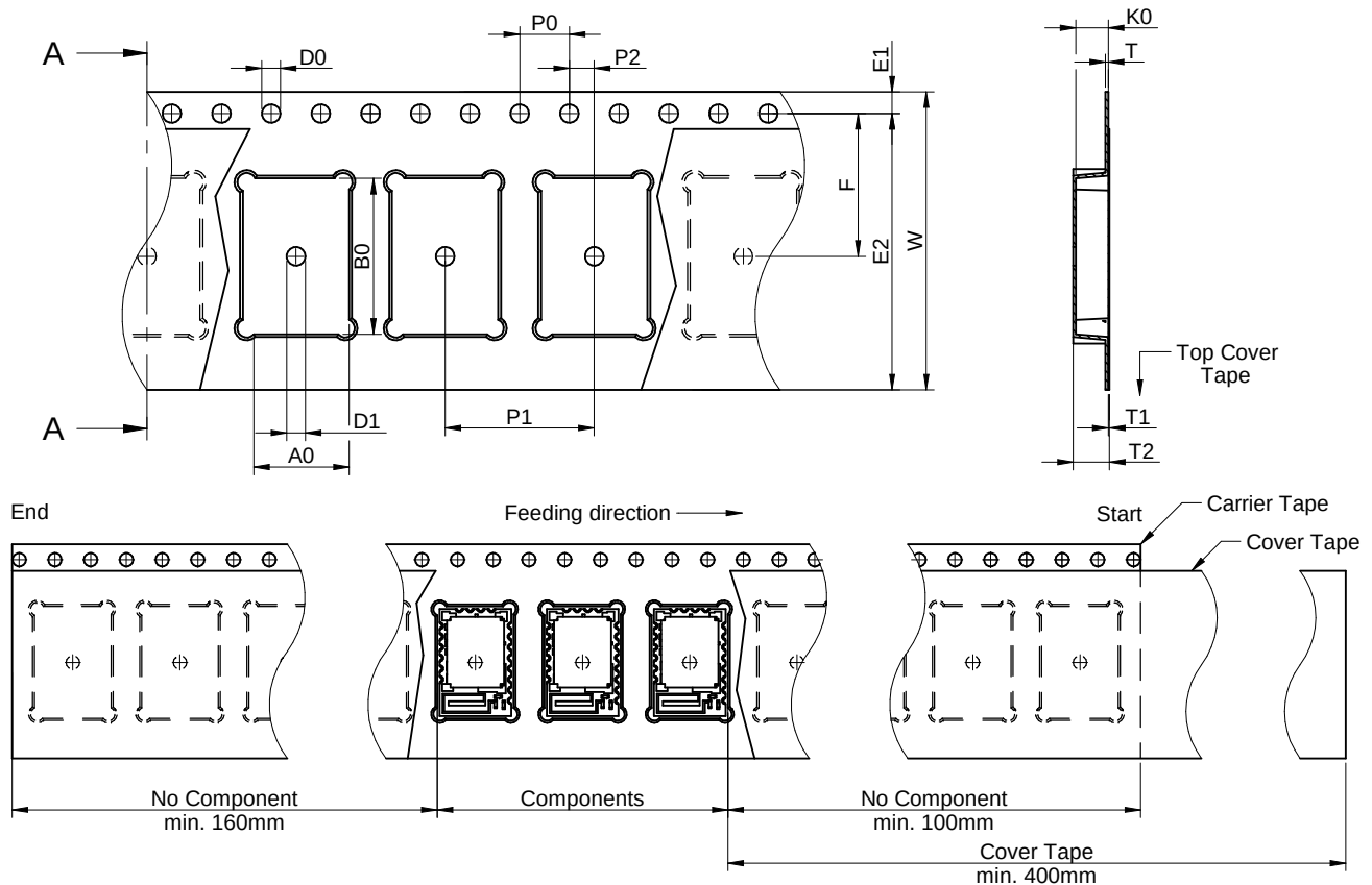
Figure 51: 24 mm Tape
